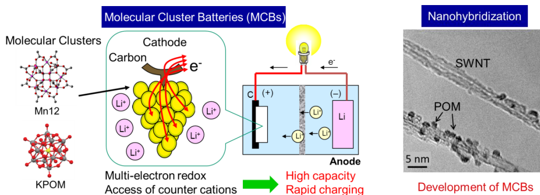
Fig.1. Schematic View of MCBs (Left) and TEM Images of Nanohybrid Materials (Right).
